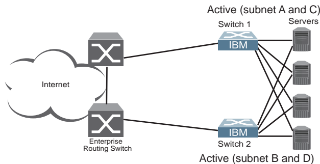
Figure 39. Active-Active Redundancy
