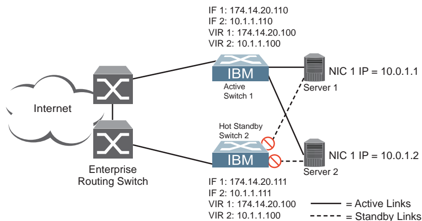
Figure 42. Hot-Standby Configuration
