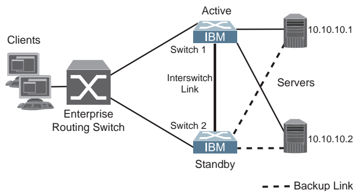
Figure 40. Hot-Standby Redundancy
