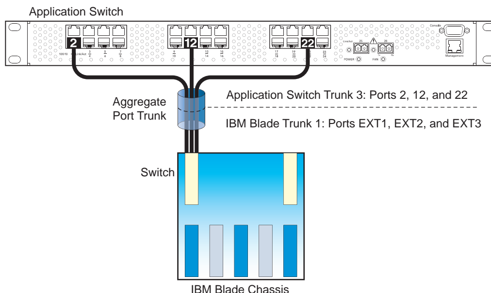
Figure 9. Port Trunk Group Configuration Example
